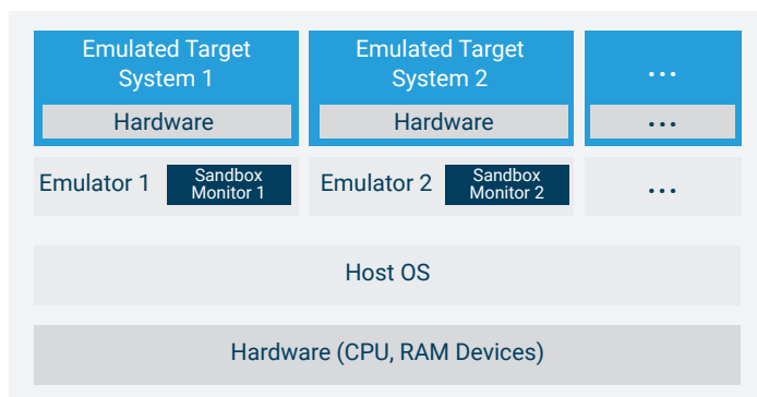
Figure 3 - In full system emulation, the CPU instruction set and memory of one CPU type can be emulated while residing in a native OS on another type of (physical) CPU
