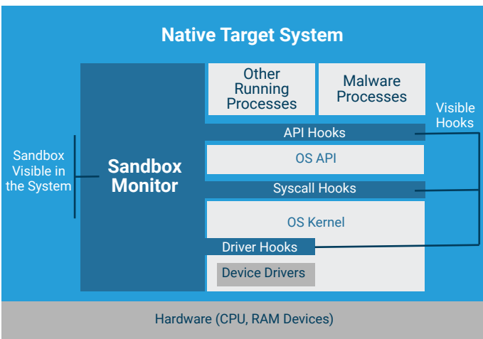
Figure 4 - Possible hooking locations in Windows
